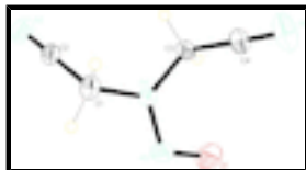
Fig. 1. Perspective drawing of the title compound with displacement ellipsoids drawn at the 30% probability level.
