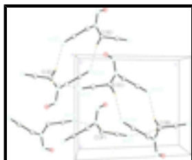
Fig. 2. The crystal packing of the title compound viewed along the a -axis showing H-bonding interactions; the H atoms not involved in H-bonds have been omitted for clarity.
